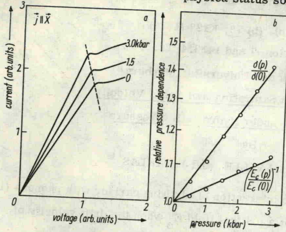
Fig. 1. I-U characteristics for \vec{j} \parallel \vec{X} at different pressures (a) and pressure dependence of conductivity \sigma and critical field E_c (b)
